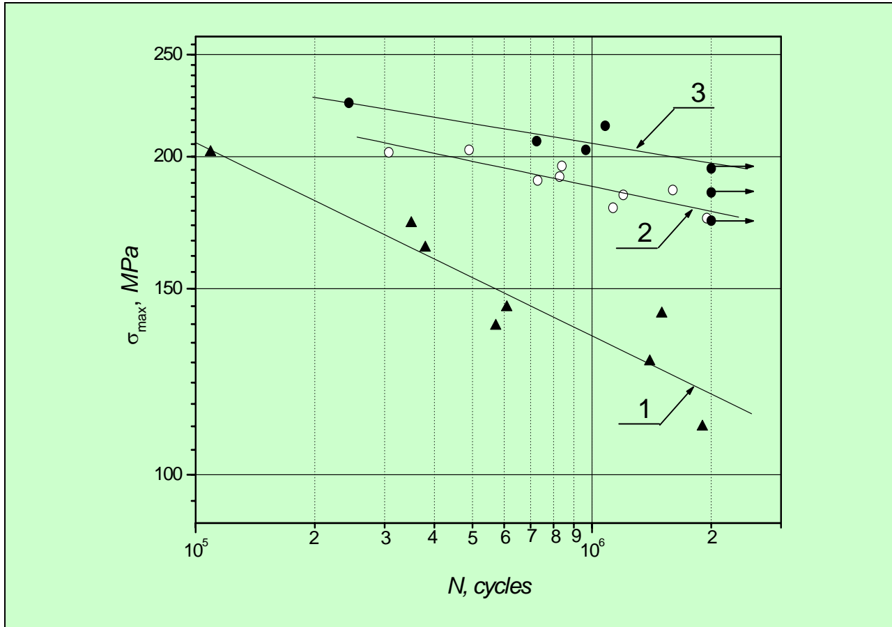
Fatigue curves of large-scale welded samples (transverse non-load-carrying attachment, R=0): 1 – in as-welded condition, 2 – UP was applied before fatigue testing, 3 – UP was applied after fatigue loading with the number of cycles corresponding to 50% of expected fatigue life of samples in as-welded condition
